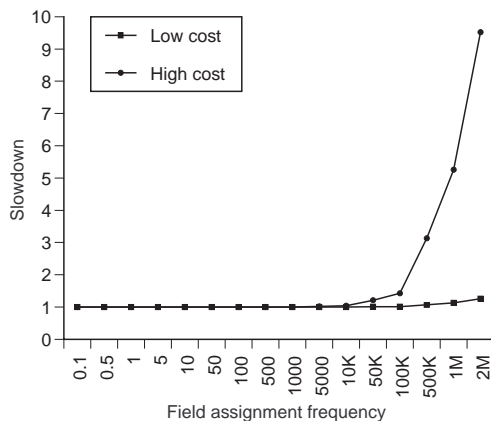
Figure 11. Predicted slowdown
